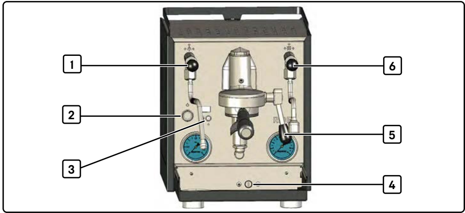
Fig. 2 Control elements
